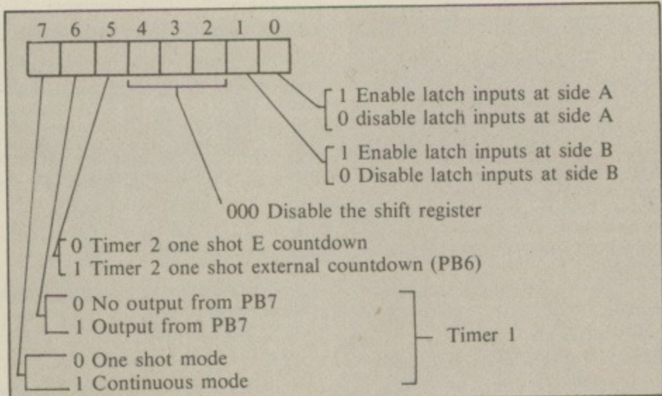
Figure I: Auxiliary control register &FE6B
