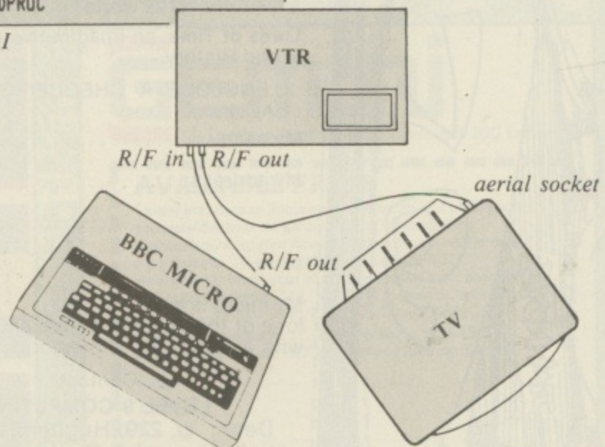
Figure 1: Connecting up the three machines
