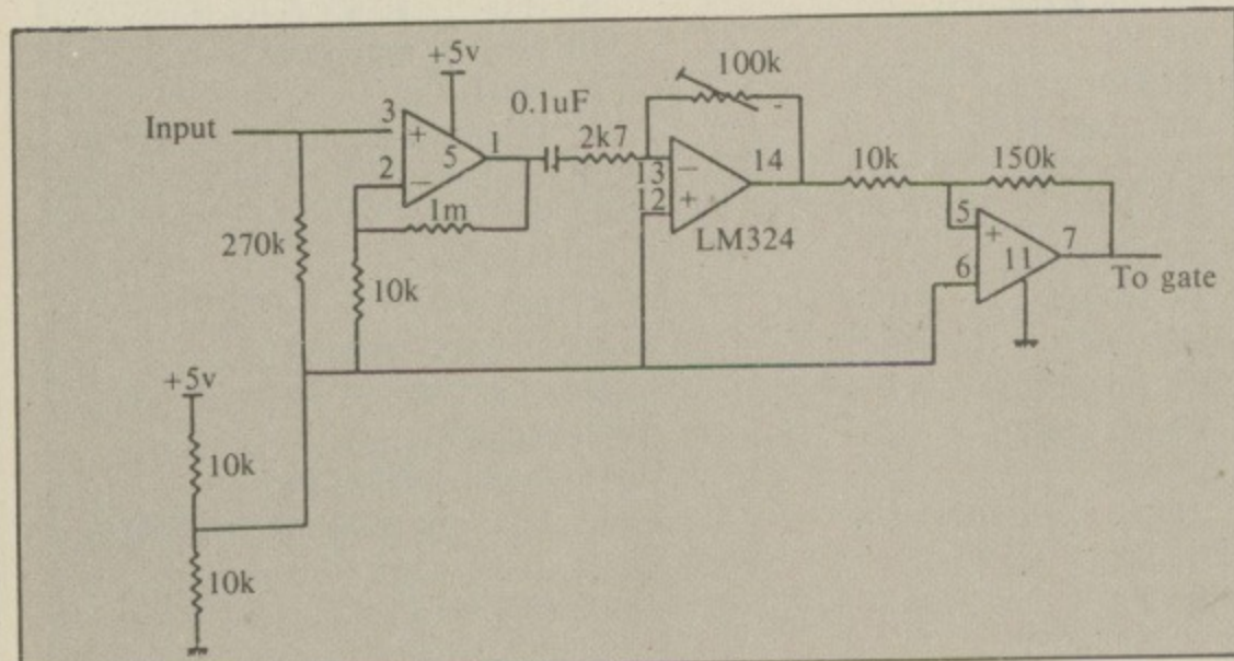
Figure III: Low level input signal amplifier
