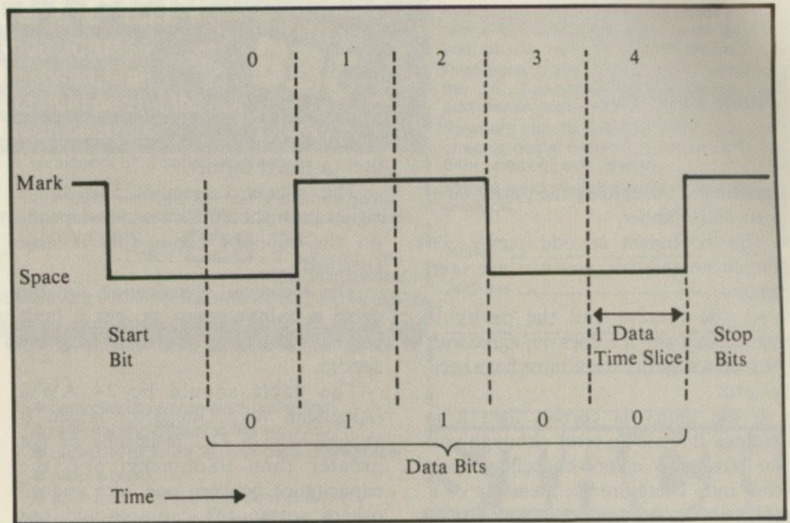
Figure 1: Asynchronous five bit data.
