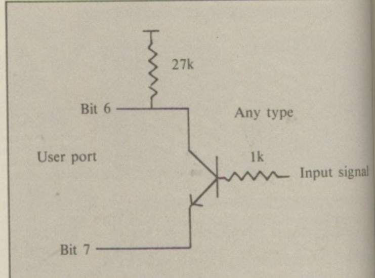
Figure II: Gating transistor
